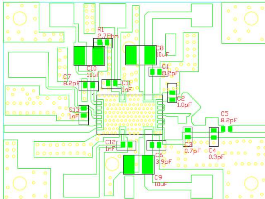
Figure 3: Picture of application board Doherty circuit for 3.4-4.0GHz
