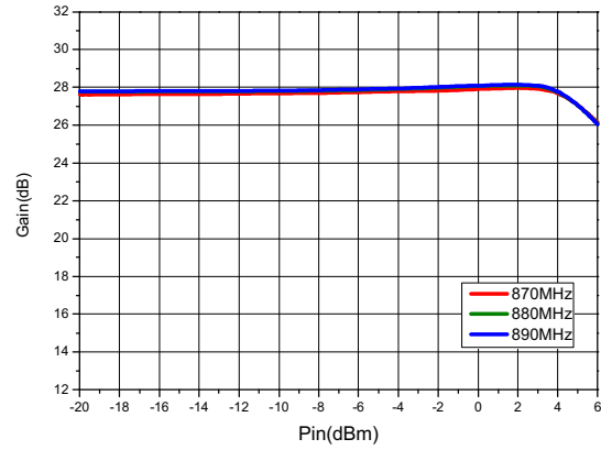
Power Gain vs. Input Power
