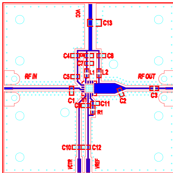
Circuit Component Designations and Values
