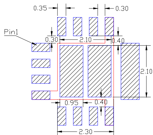
Combined PCB Land Pattern and Stencil Outline
