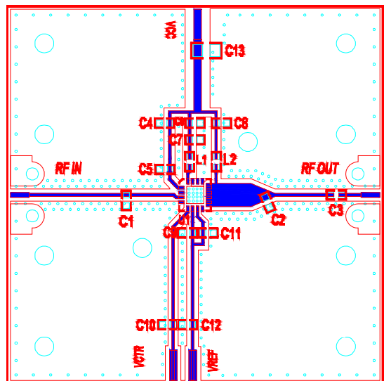
Circuit Component Designations and Values
