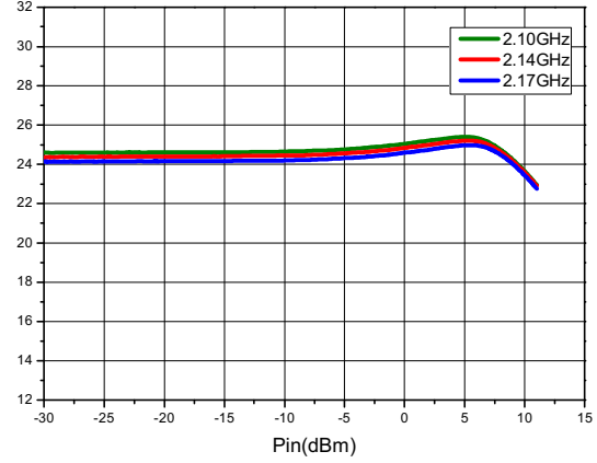
Power Gain vs. Input Power
