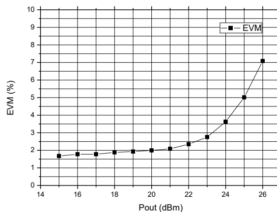
Figure: 802.11a 64QAM EVM vs Output Power @6.0GHz VR=2.9V
