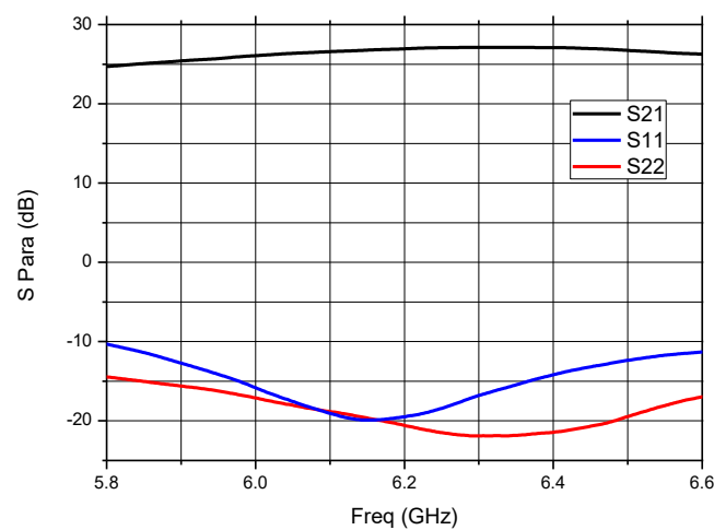
Figure: 5.9-6.5GHz Small Signal Parameters @VR=2.65V ICQ=180mA
