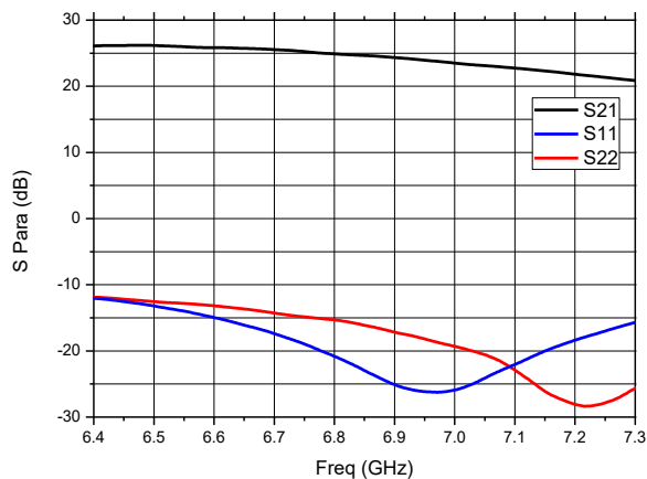
Figure: Small Signal Parameters @ V_R=2.65V I_{CQ}=180mA
