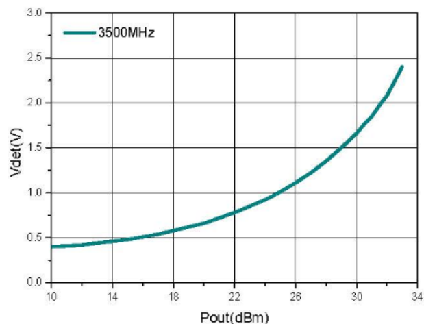
Vdet vs. Pout
