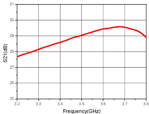
S21 vs. Frequency
