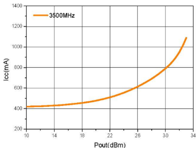
Icc vs. Pout
